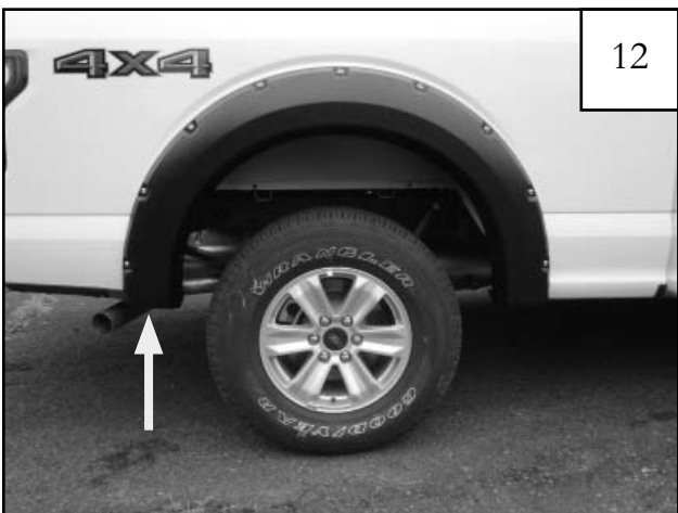
Install supplied push retainer (RV1-P0006) into flare and through factory hole at rear of wheel well.
