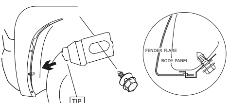
LEVER CLIP + SCREW W/WASHER
