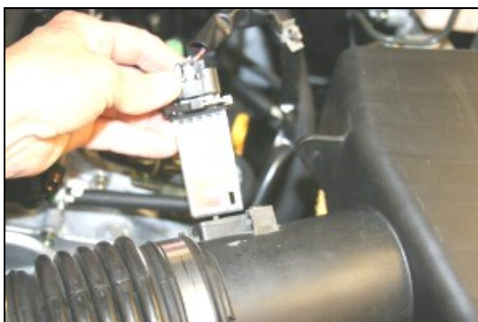
5. Without disconnecting the MAF sensor, remove it from the factory airbox lid, and set it aside. It is important to note the direction of the MAF sensor when removed, as to assure correct reinstallation later in the install process. The MAF sensor must be installed in the correct direction for proper air flow calibration.
