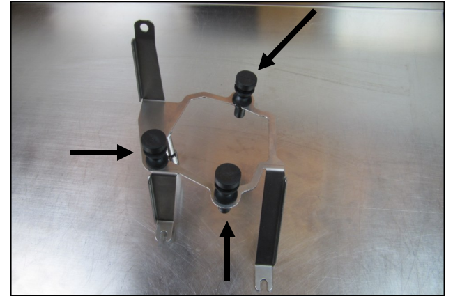
28. Transfer the three rubber air pump mounts from the factory bracket into the Airaid Air Pump Bracket (#6) and re mount the pump.
