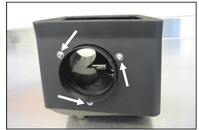
34. Mount the Filter Adapter (#5) to the Cold Air Box, as shown, using three 1/4-20 x 1/2" Button head Bolts (#18) and 1/4" Flat Washers (#19).
