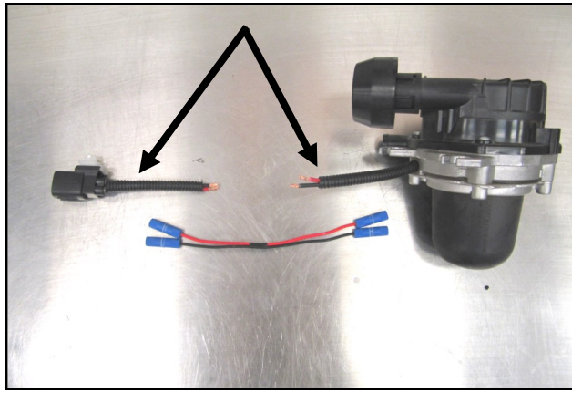
21. Cut 1 inch from each piece of the factory wire loom and re install onto the pump and connector wires.
