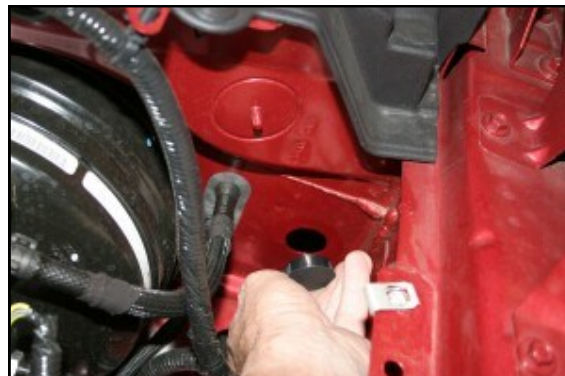
7. Install the optional firewall plug (#19 on the main page) into the hole in the firewall.
