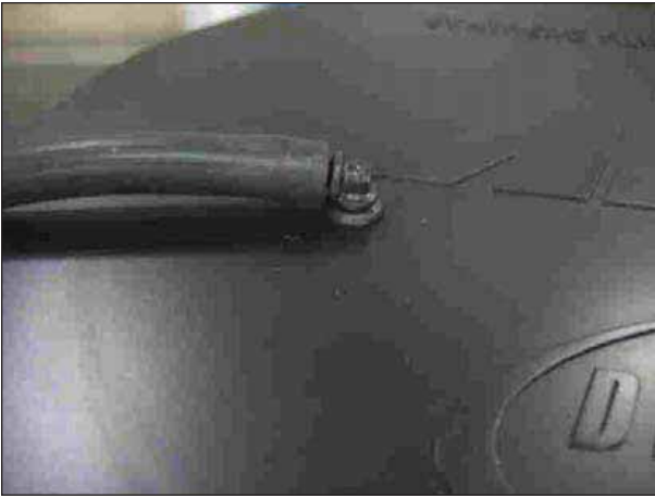
e. Push one end of 5/32" elbow into grommet. Again, you may want to use soapy water to lubricate grommet.
