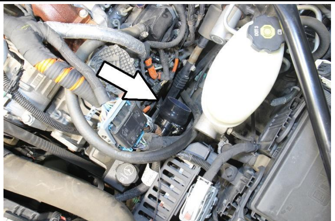
25. Carefully, insert the hot side charge pipe to the intercooler inlet.
