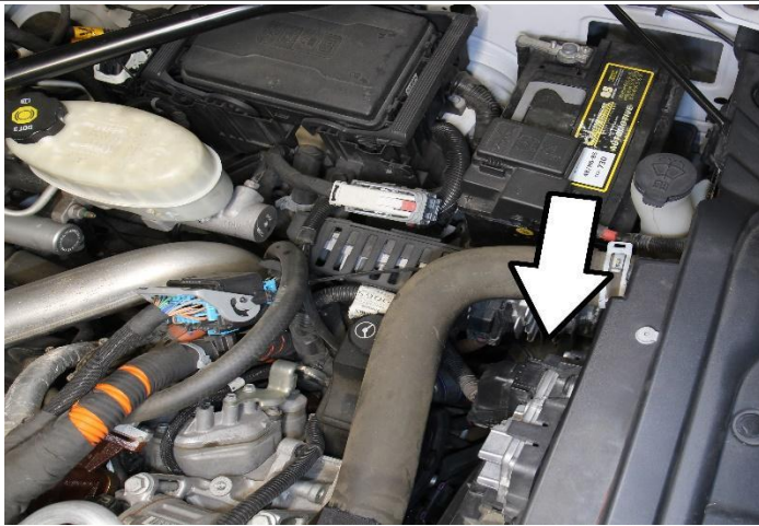
20. In this case, the hose clamp was facing the top of the engine. Loosen the hose clamp securing the charge pipe to the intercooler from the top of engine using a long extension.
