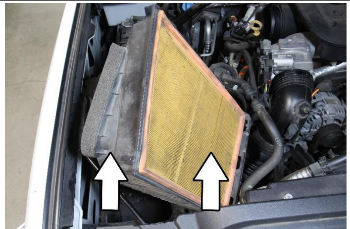
7. Lift up gently and disconnect the lower air box assembly from the rubber grommets. Remove the lower air box assembly from the vehicle.
