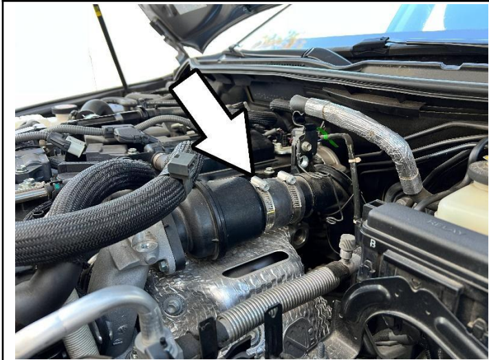
9. Loosen the hose clamp securing the intercooler hose from the turbo resonator.
