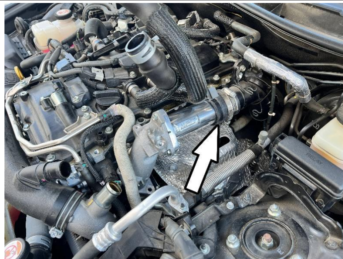
16. Insert the resonator delete pipe into the intercooler hose first, then onto the turbo housing.
