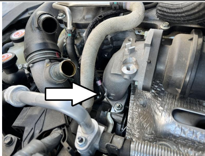
11. Unclip the vacuum hose from the turbo outlet elbow.
