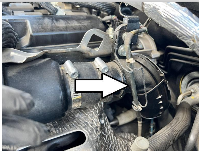
5. Disconnect the O2 sensor harness from the bracket.
